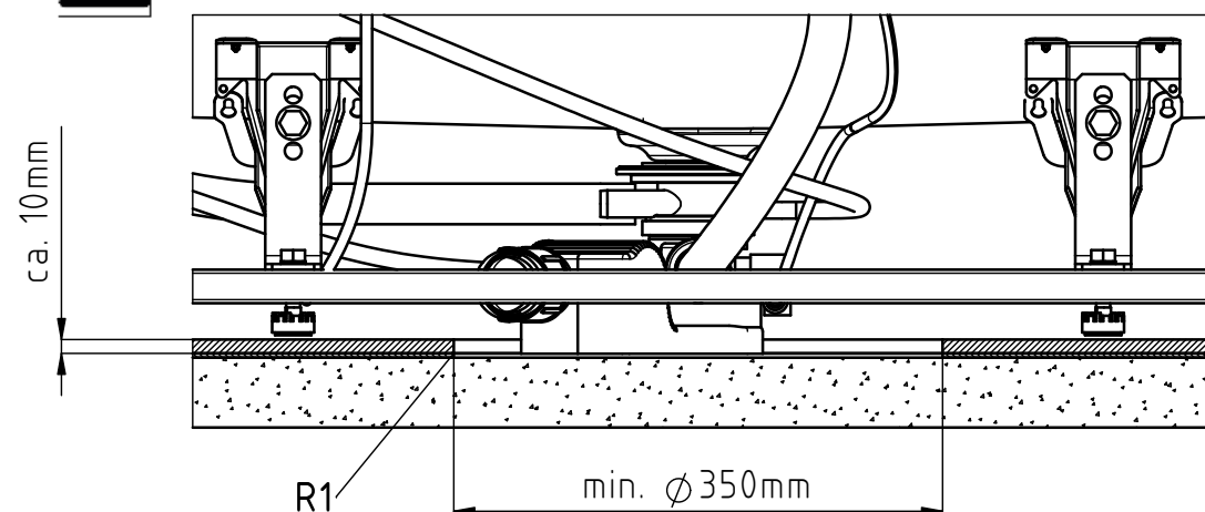
DETAIL A
