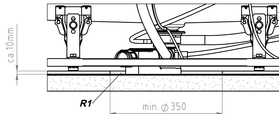
DETAIL A
