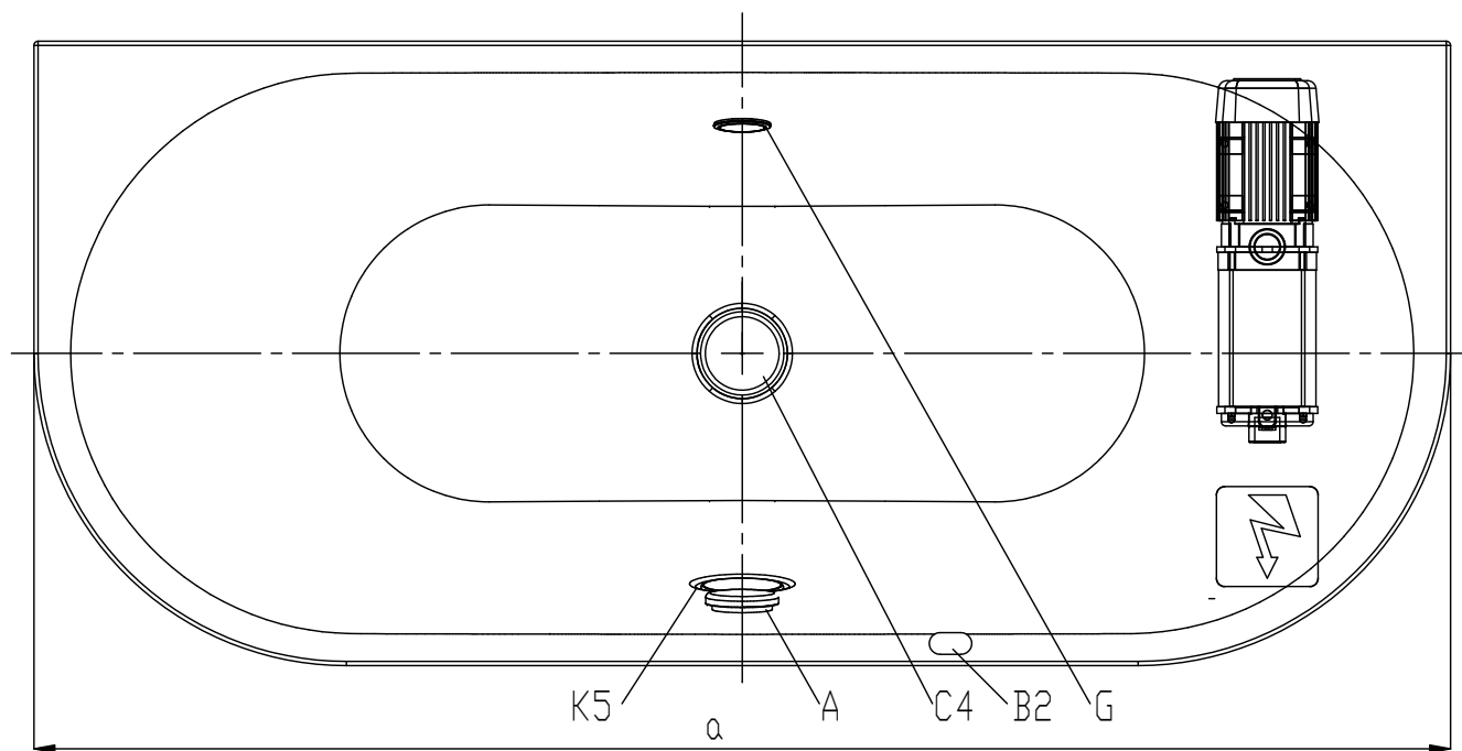
DETAIL A
