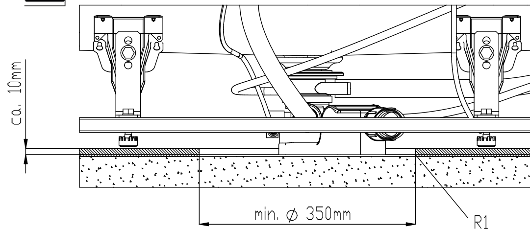
DETAIL A
