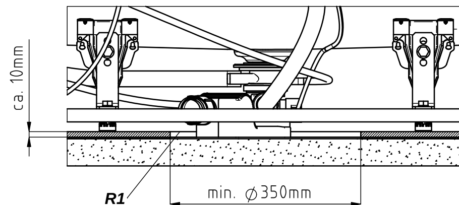
DETAIL A
